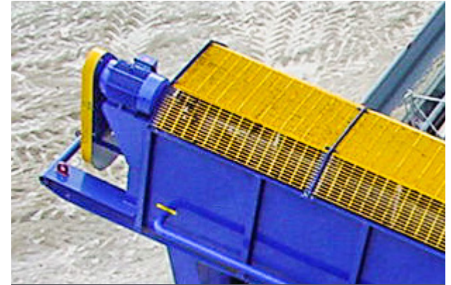
PERSONAL SAFETY COVERS AND GUARDING
